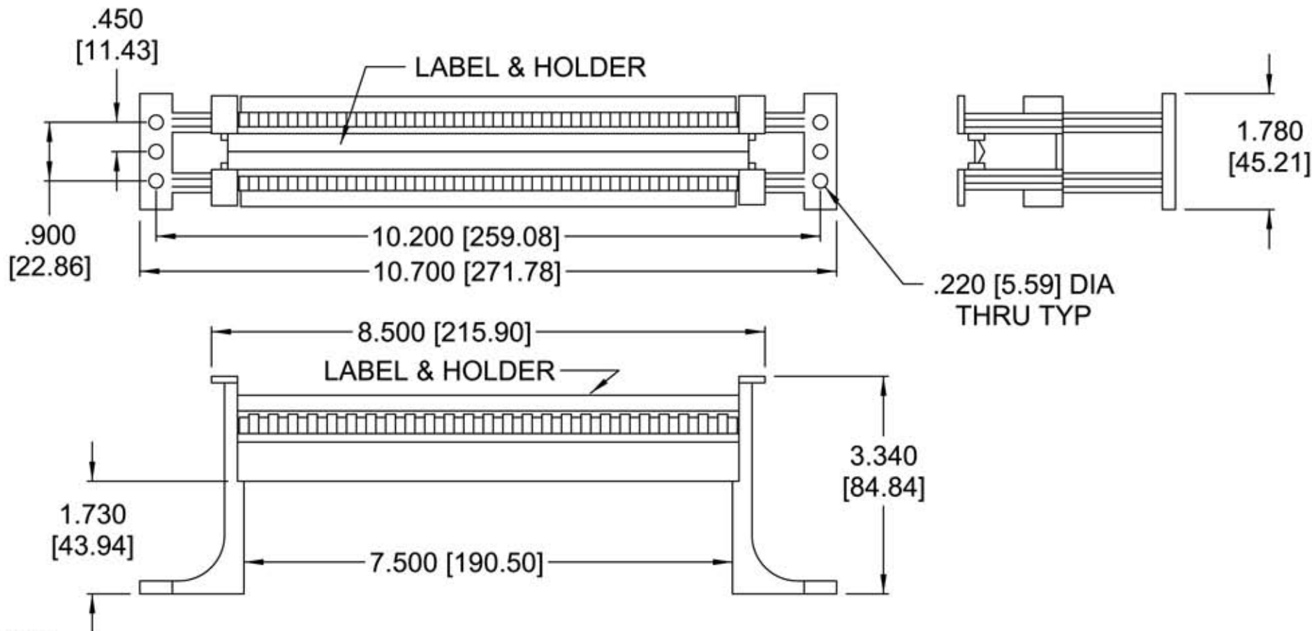
LABEL & HOLDER DETAIL
